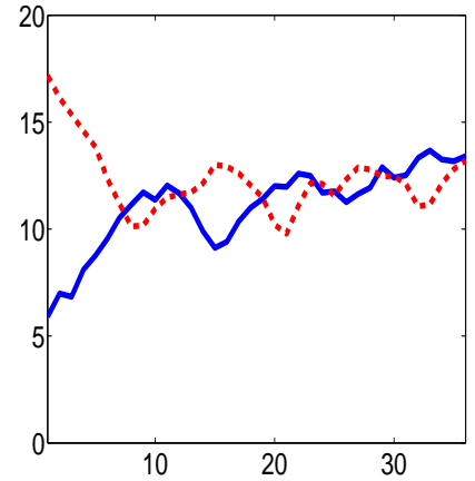
Panel D: Return on equity, r_{it+1}^S
