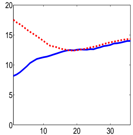
Panel H: Return on equity, r_{it+1}^F
